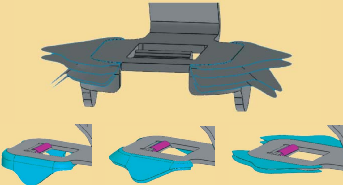
MULTIPLE STEP UNFOLDING OF FLANGE FEATURE
