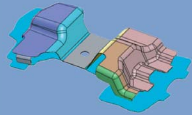
UNFOLDING BEND CORNER
