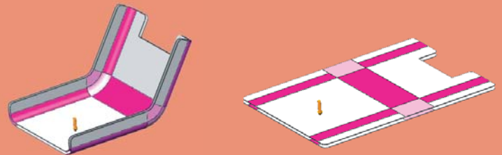
UNFOLDING BEND CORNER
